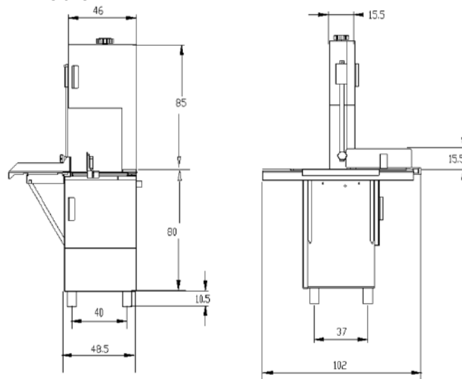
FIG. 9 MEATSAW GENERAL DIMENSIONS
