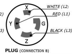
PLUG (CONNECTION B)
