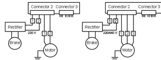
FIG. A2 CONNECTIONS SINGLE PHASE
